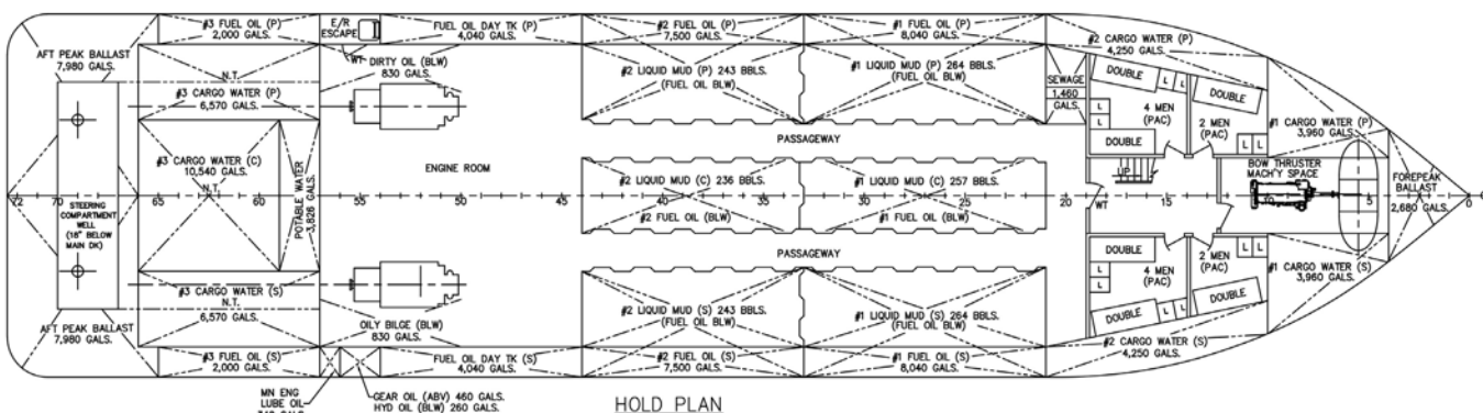
HOLD PLAN
