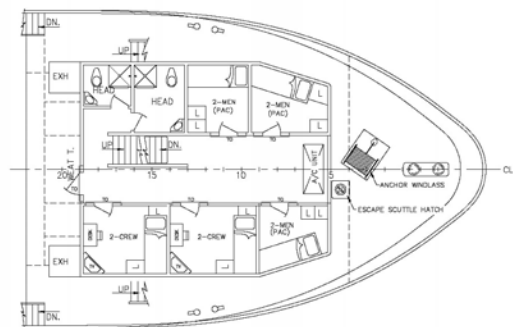
FOC'SLE DECK
