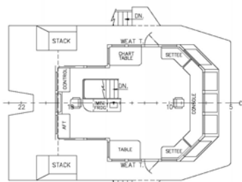
PILOT HOUSE
